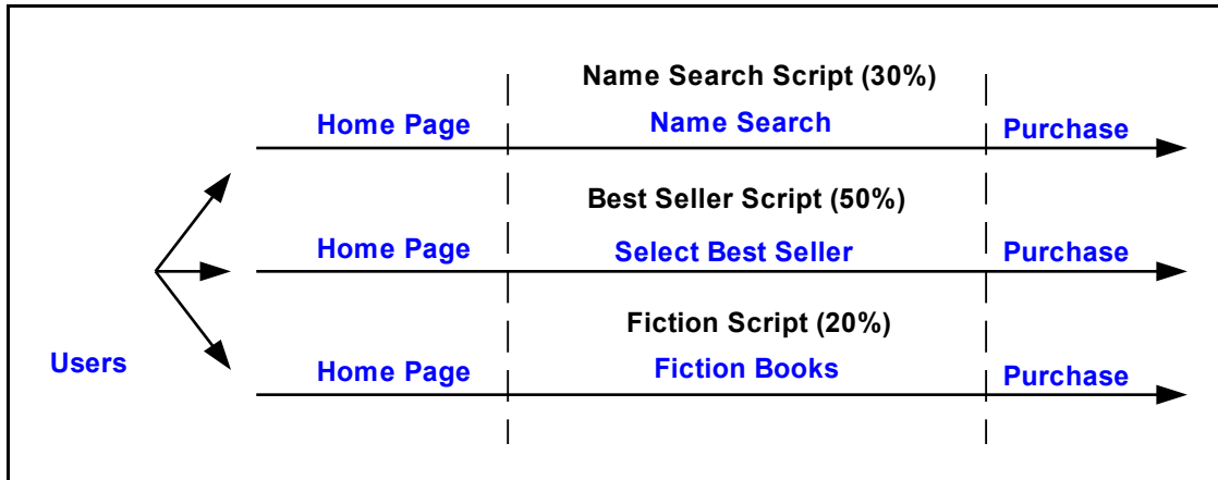
Figure 2: Using entire-path scripts to represent the “choose a fiction book” paths
