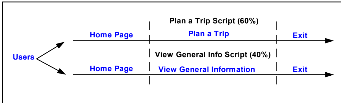
Figure 8: Entire-path scripts for representing WMATA user paths
