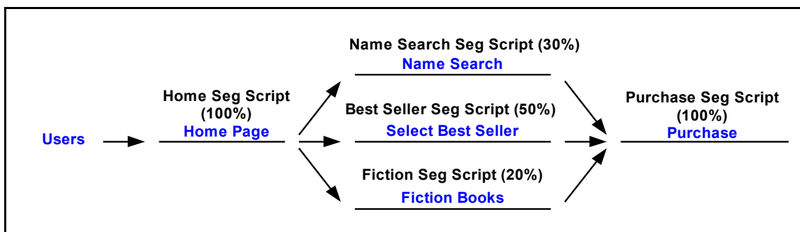
Figure 4: Using split scripts to represent the “choose a fiction book” paths
