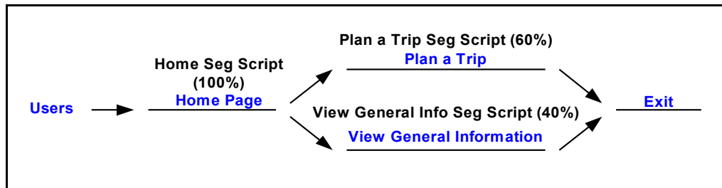
Figure 10: Split scripts for representing WMATA user paths
